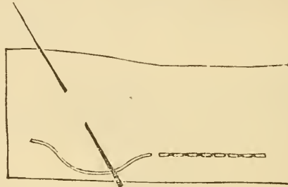
Stitching.
